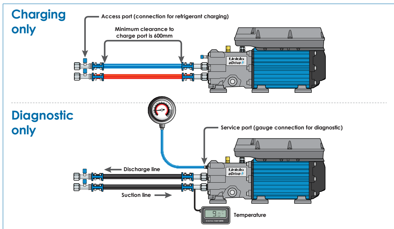
Refrigerant charging and diagnostic access points
