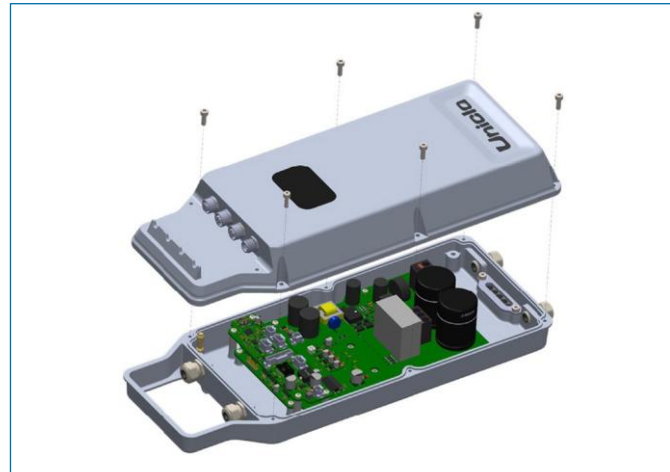
Electrical enclosure (controller housing) access
