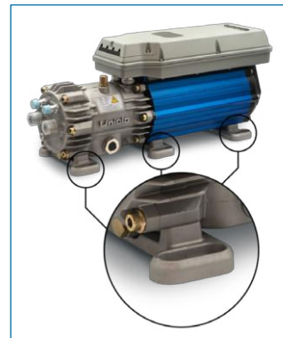
Mounting points (x6)
