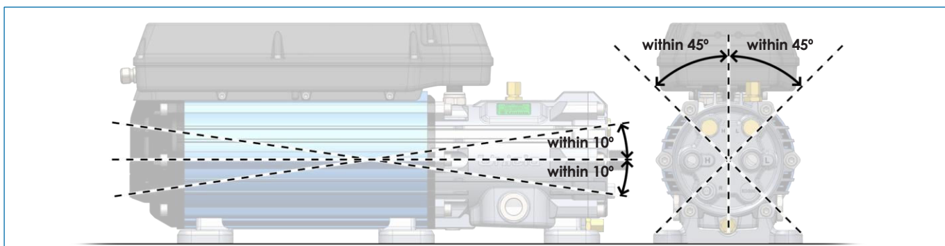
Mounting angle
