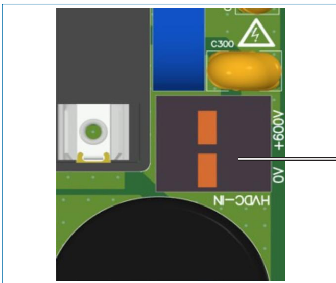
Vdc connection
