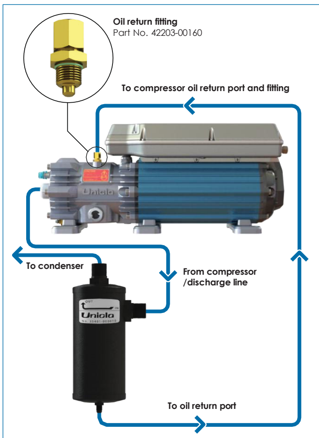
Connection options for Unicla oil separator
