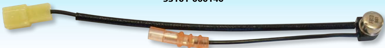
Thermal switch to suit rear manifold (32308-000760) setting cut out 95°C - cut in 75°C 53101-000140
