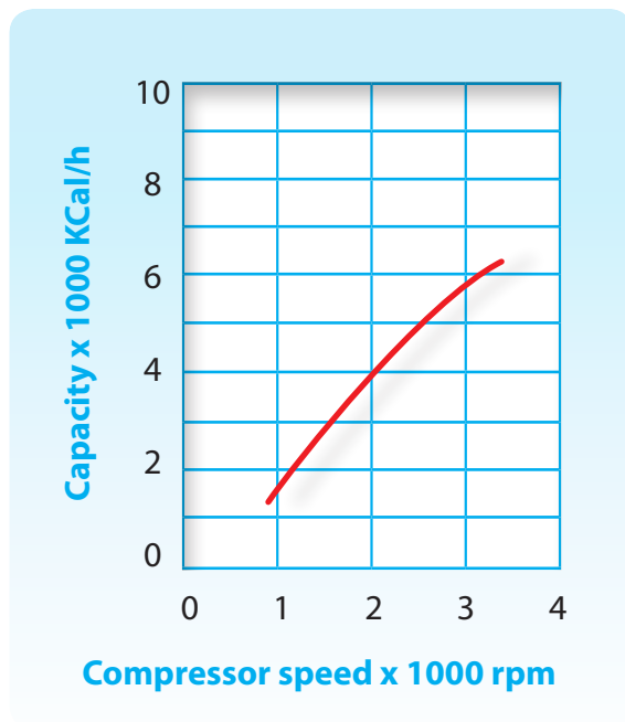
Graph 4. Compressor performance 1.
