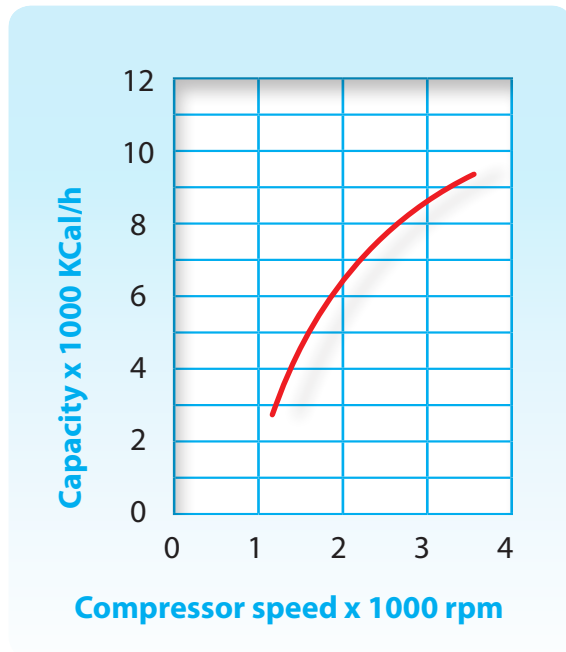
Graph 5. Compressor performance 2
