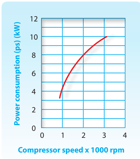
Graph 6. Compressor 1 performance
