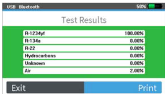
Figure 17 Percentage of Air Present
