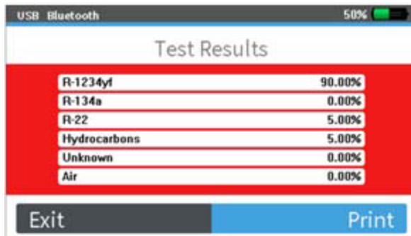
Figure 16 Refrigerant Sampled is < 95% Pure
